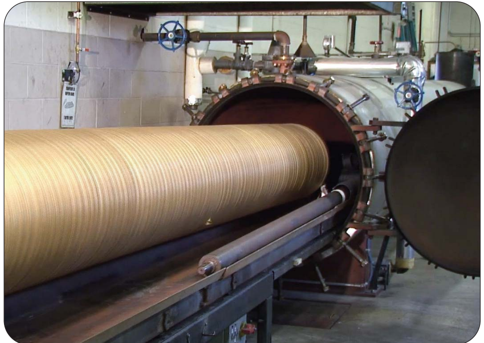
Rubber hose vulcanizing process
