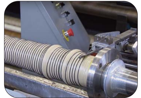
Automated helical wire winding process
